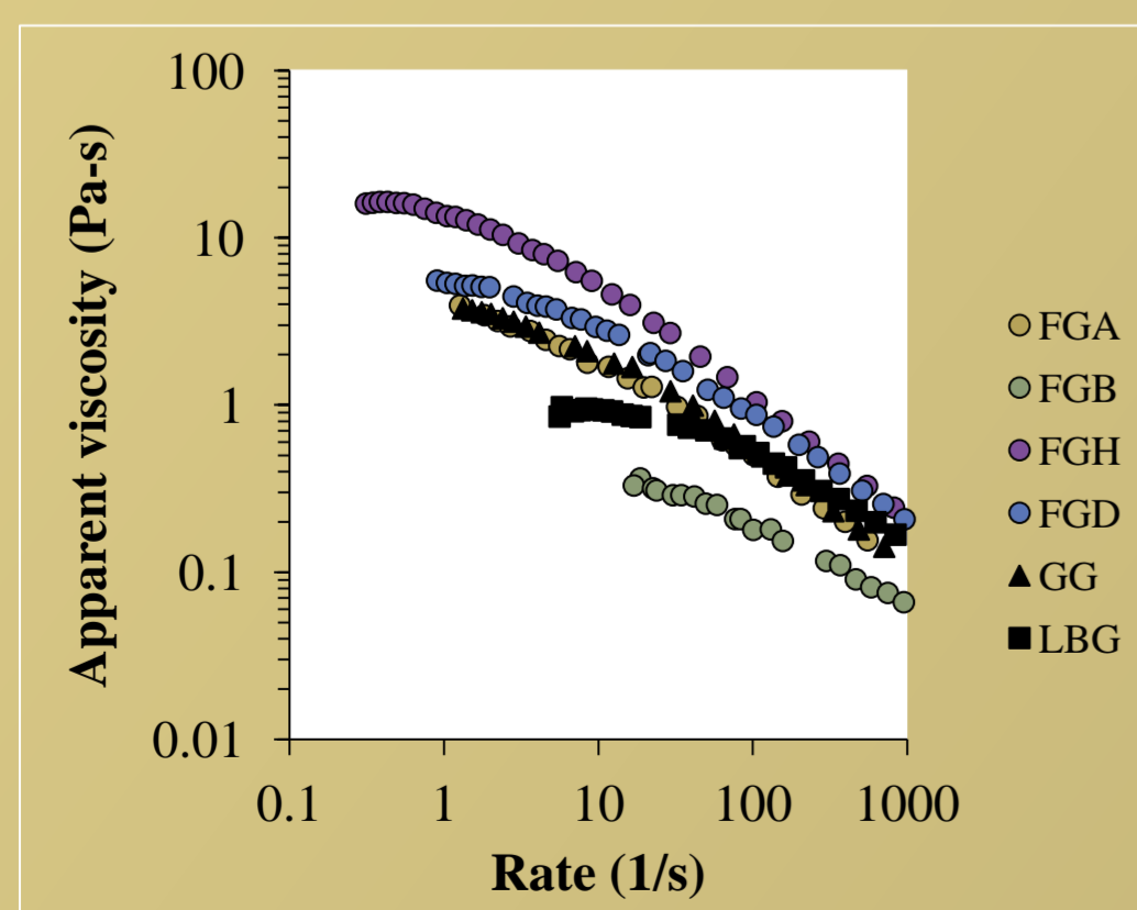
Figure 1: Apparent viscosity of 1% galactomannan solutions.
